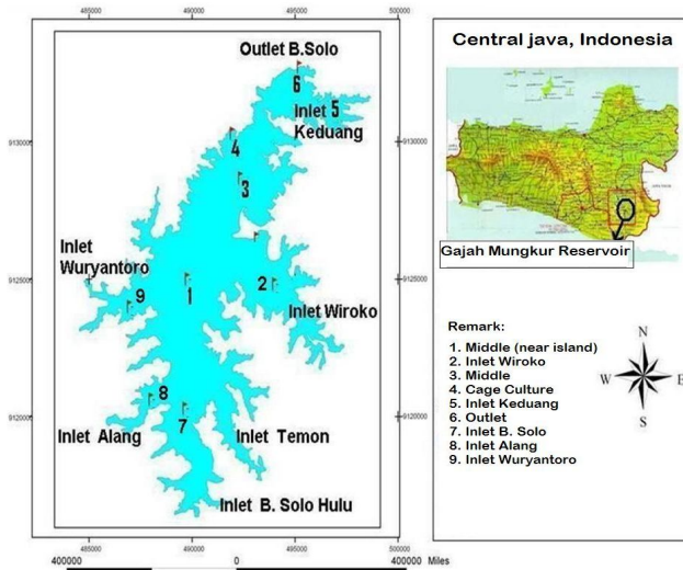
Figure 2. Location Site Map of Sedimentation Sampling
