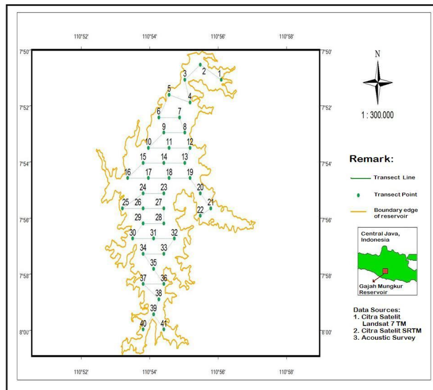
Figure 1. Acoustic transects design in Gajah Mungkur Reservoir
