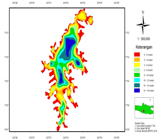
Figure 3: Bathymetry Map of Gajah Mungkur Reservoir
