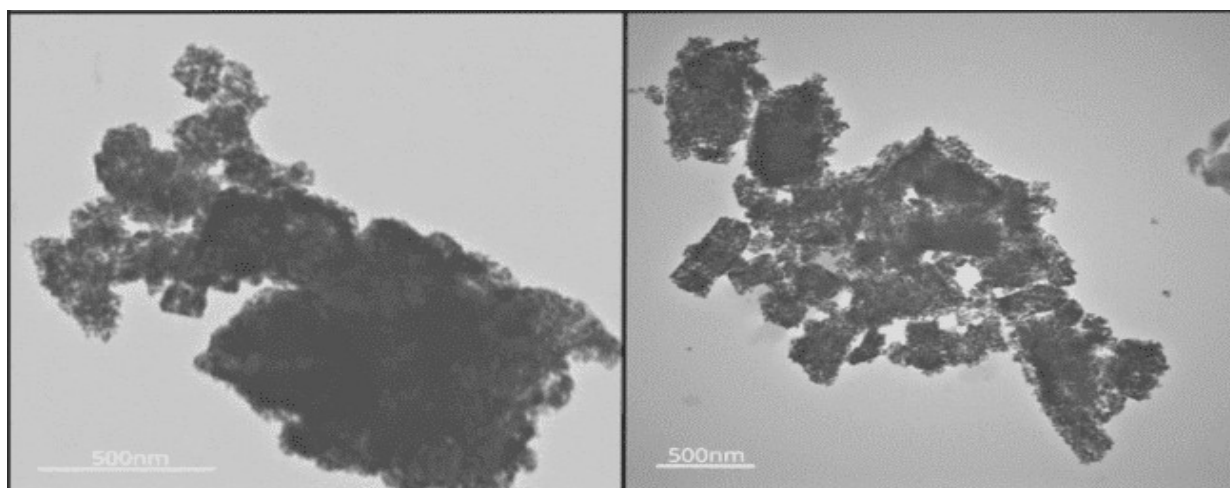
Figure 1. STEM images from sample B1
