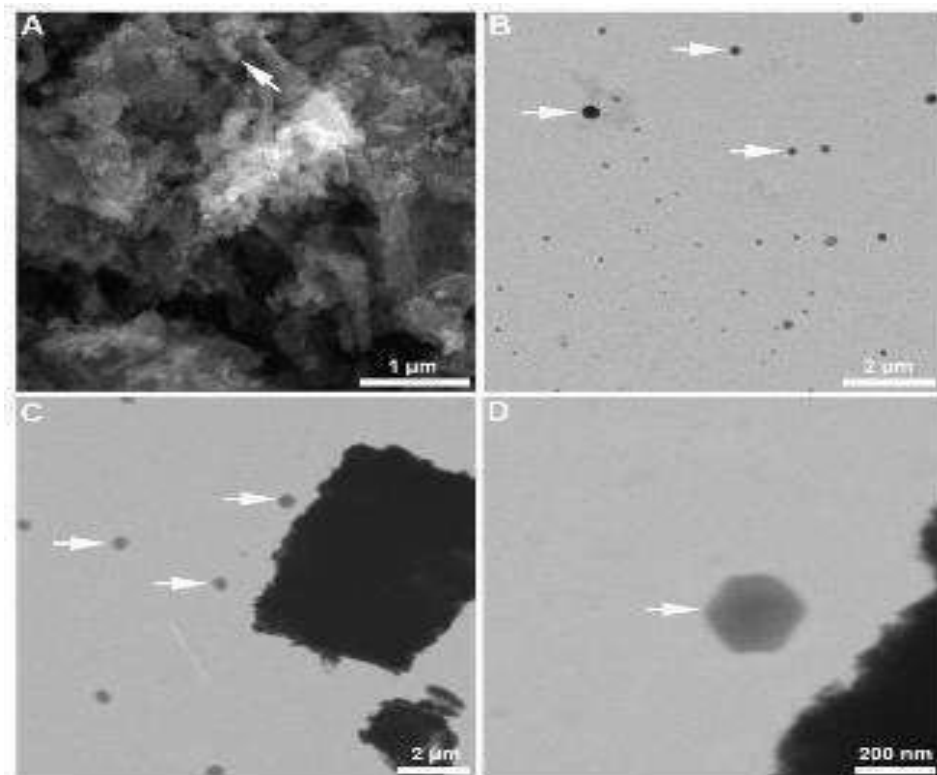
Figure 3. STEM images from sample B3
