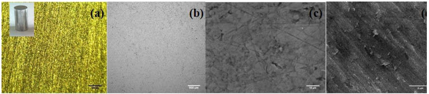
Fig. 2. Optical image of polished non-etched surfaces at 400x magnifications for 1.0 wt% rGO-AMNC (a) and SEM images under different magnifications (b-d) for 1.0 wt% rGO-AMNC
