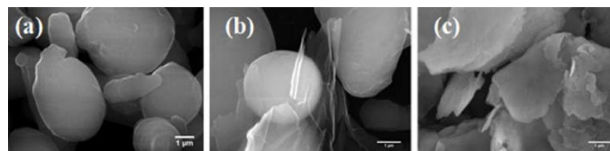
Fig. 1. SEM images of Al particle(a), 1.0 wt% rGO-AMNC before dispersion (b) and 1.0 wt% rGO-AMNC after ball milling dispersion (c)
