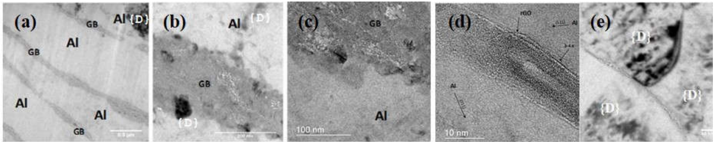
Fig. 3. TEM images under different magnifications for the 1 wt% rGO-AMNC sample
