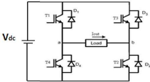
Fig .1. single phase full bridge inverter
