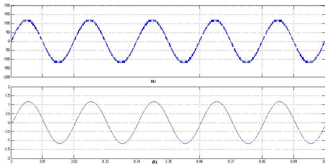
Fig. 3. (a) Output voltage waveform (b) Load current waveform
