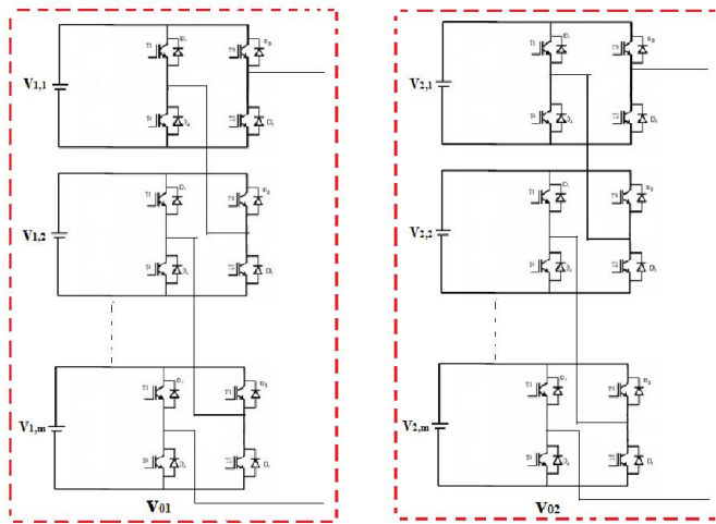
Fig. 2. Cascaded sub-multilevel inverter
