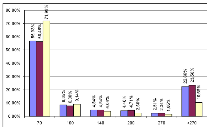
Fig. 4 Graph showing the comparison of the particle size distribution of the primary milling (red and blue) and the second milling (yellow) (Souza et al., 2016)
