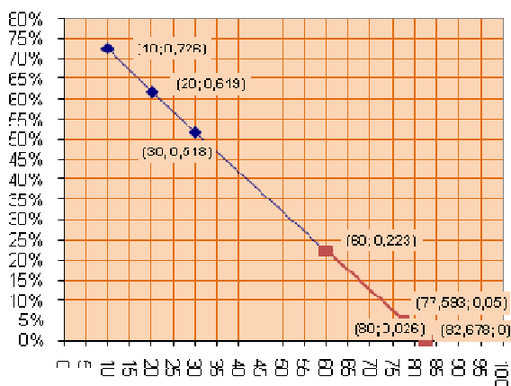
Fig. 2 Time Analysis for definition of Work Index: X-axis: time in minutes; Y-axis: % pass by (Souza et al., 2016)
