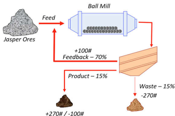
Fig. 5. Flow chart of selective milling (Souza et al., 2016)
