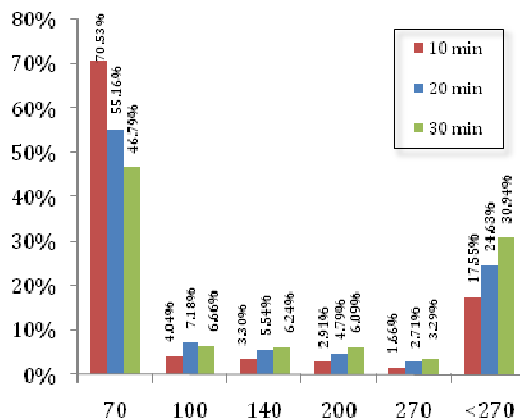
Fig. 3 Comparative graph of the effect of milling time on the comminution of the samples (Souza et al., 2016)
